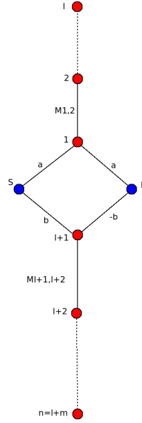
Figure 8. Canonical realisation for auto-reciprocal responses - upper antenna contains l resonators and lower one m
