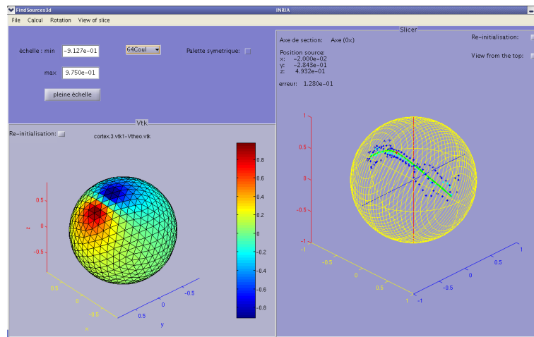
Figure 4. Views of the potential for one source and of poles on plane sections in FindSources3D
