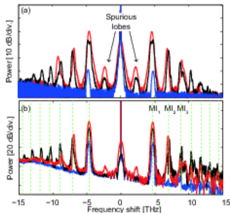
Figure 2. Experimental (above) and numerical (below) gain for the modulational instability in (periodic) optic fibers
