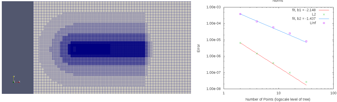
(a) Example of QuadTree mesh for circular cylinder (b) Norms as a function of number of points on grid Figure 18.
