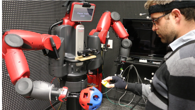
Figure 16. Representation of the setup considered in the user study. The robot presents to the user a spherical ball in which multiple shapes can be inserted. Final pose of the object is calculated from the user posture at his current location. Body motions during the insertion are recorded using a suit made from OptiTrack markers.
