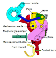
(a) Circuit breakers mechanisms [40]
